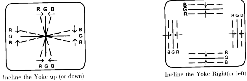
Circumference Convergence by DEF Yoke
